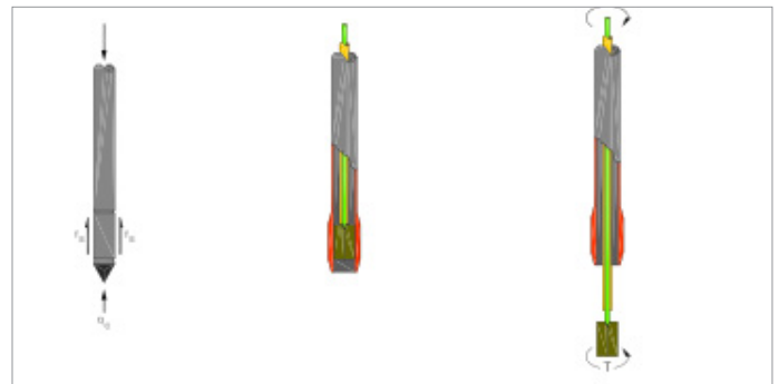
Left to right: normal cone, in situ vane, in situ vane deployed
