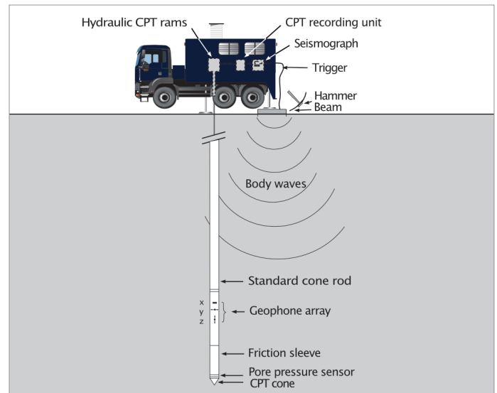
Reliable, cost effective technique to determine in situ seismic wave velocity
