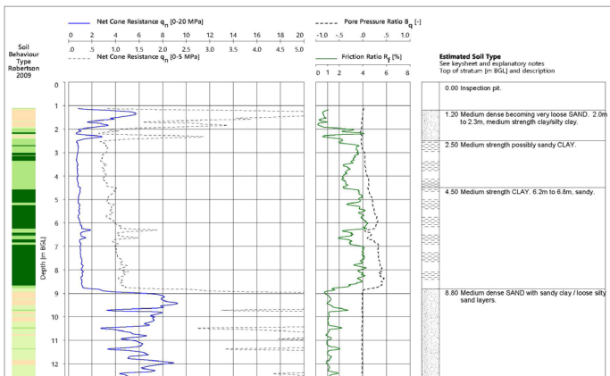
Cone resistance versus sleeve friction results into soil type classification
