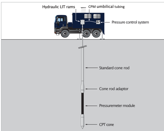
Reliable measurement of the in situ strength and load deformation behaviour of the soil
